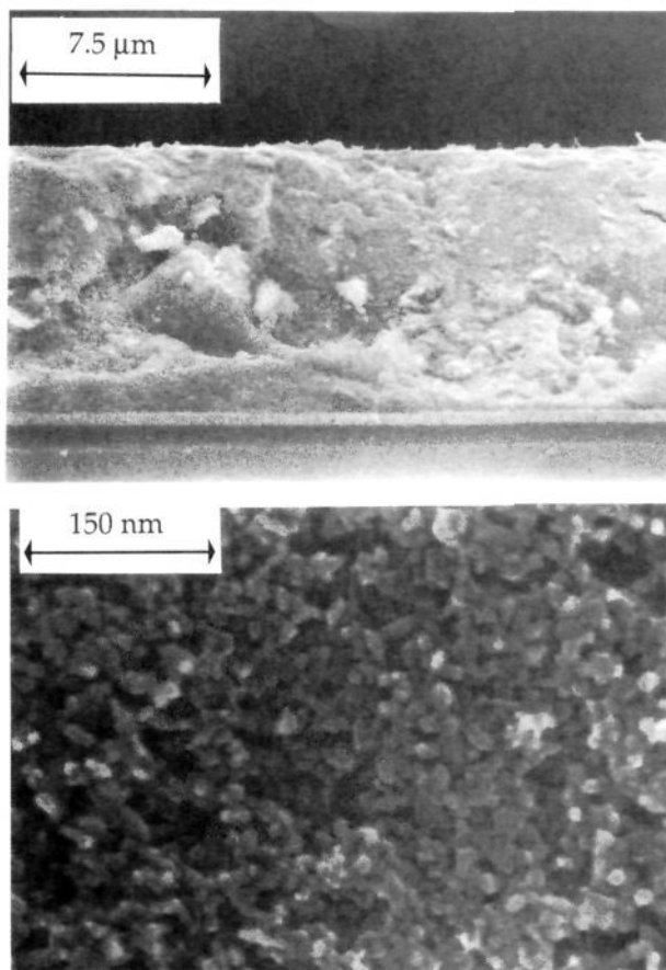
Figure 1. Scanning electron micrograph showing cross sections of the \text{TiO}_2 films deposited on conducting glass: top, low resolution and bottom, high resolution. Scales indicated on the photographs. Thickness of \text{TiO}_2 film was 10.4 \mu\text{m} ; film was prepared by Method A.
