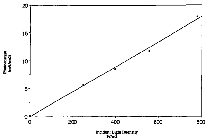
Figure 7. Effect of light intensity on the short-circuit photocurrent of the cell. Conditions: electrolyte as in Figure 5, TiO_2 surface treated with 4- tert -butylpyridine before being wetted with electrolyte, room temperature, AM 1.5 spectral irradiance.
